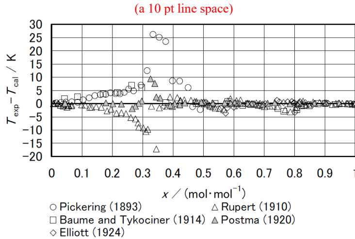
(a 10 pt line space) Fig.1 Deviation of measured freezing point temperatures from correlations by Tillner-Roth [2]. (a 10 pt line space)
